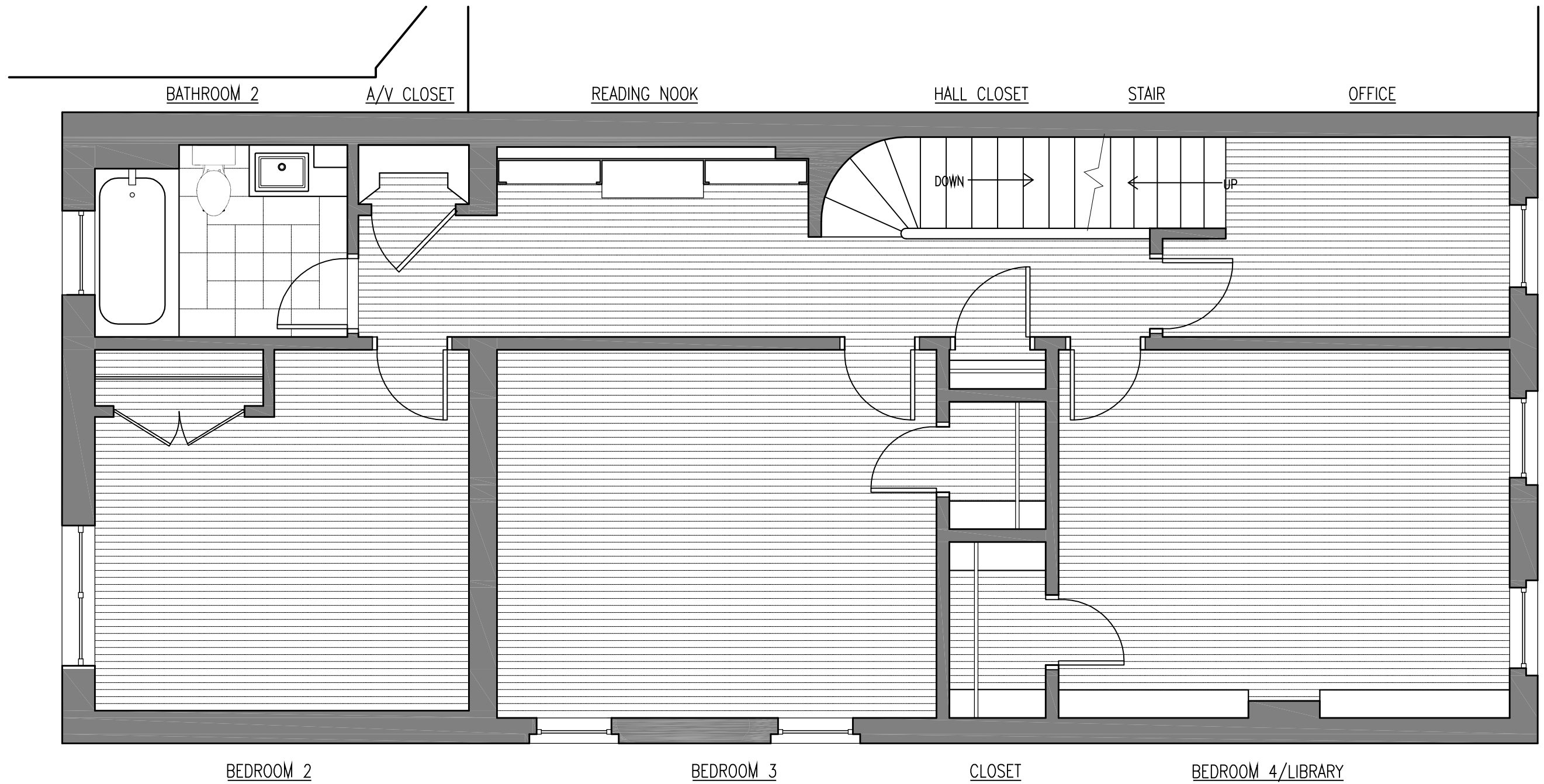
THIRD FLOOR PLAN N ►
