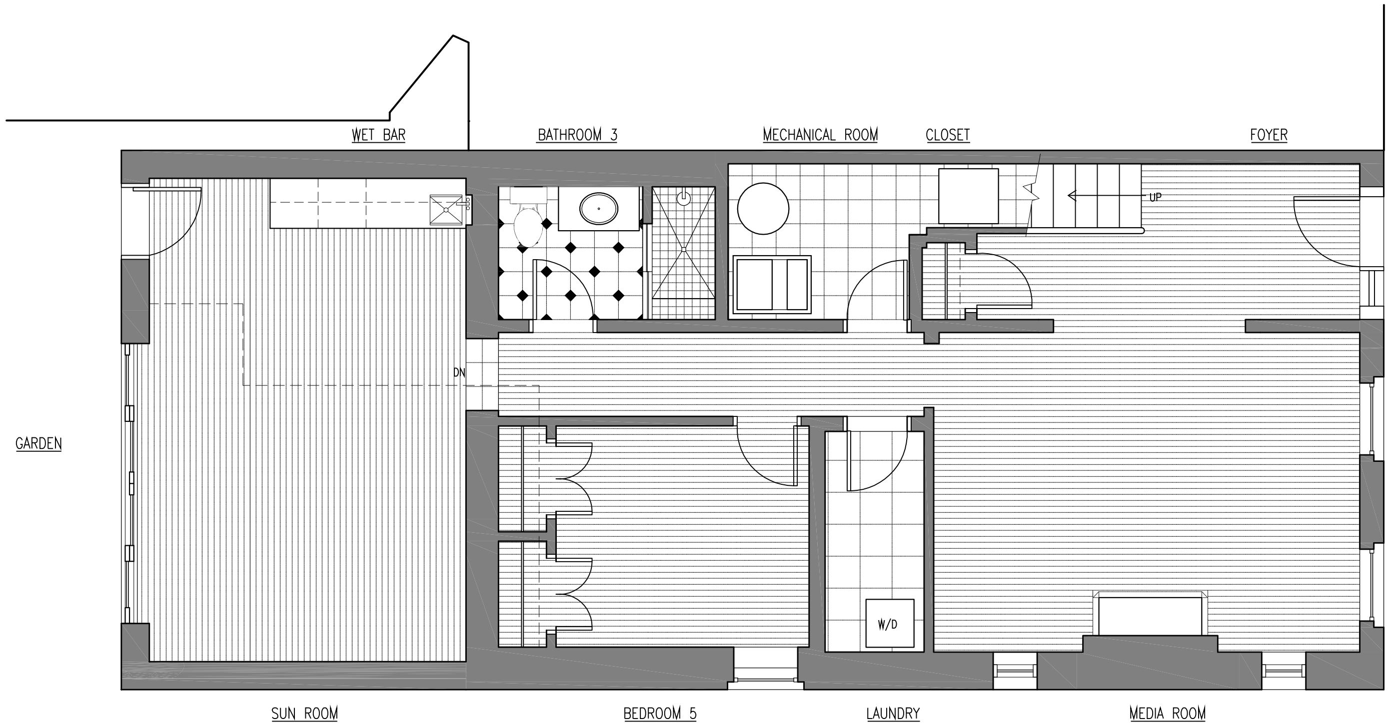
FIRST FLOOR PLAN N ►
