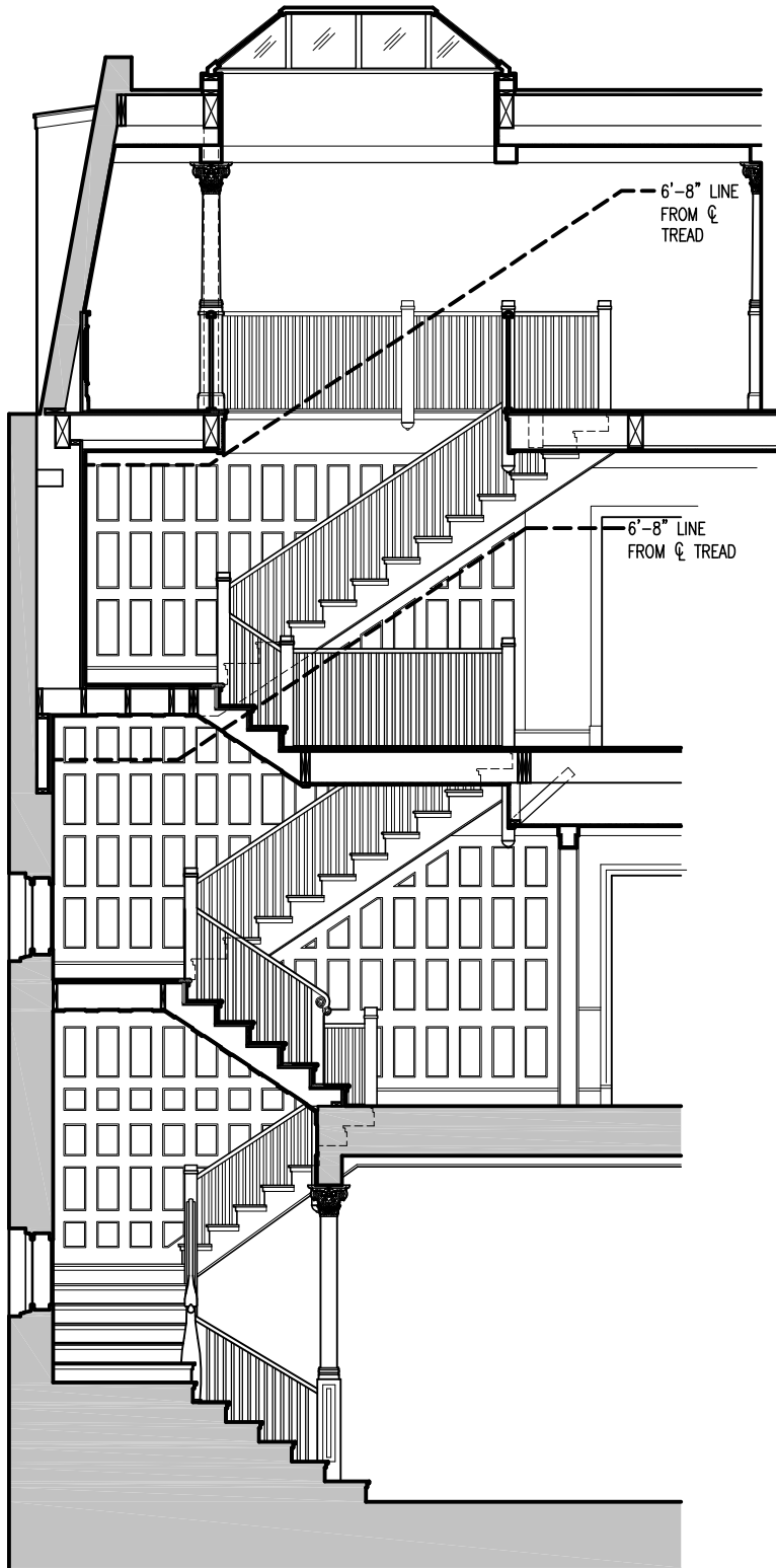
STAIR SECTION
